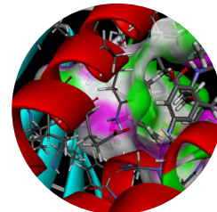
Crystal structure superimposed on Hsp90 (1OSF) docked 17-demethoxy geldanamycin derivative.
